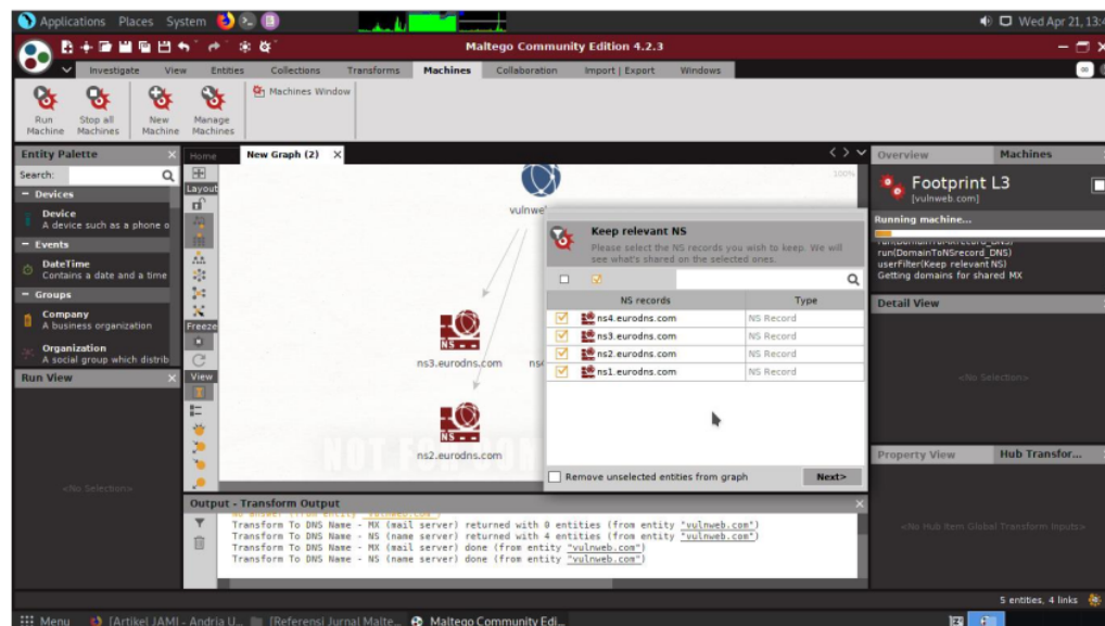
Gambar 4. Proses Footprinting
